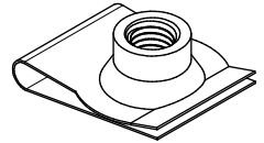
Barrel Nut 3/8"-16 UNC Qty 24
