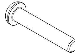
BUTTON HEAD SOCKET CAP SCREW BLACK OXIDE M8 x 1.25 x 45 mm QTY 4
