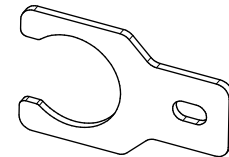
MB2117-01 Park Sensor Retainer Plate Qty 4
