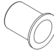
Rivnut 5/16"-18 Qty 14
