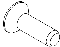
COUNTERSUNK SOCKET CAP SCREW 5/16"-18 x 1" Qty: 14
