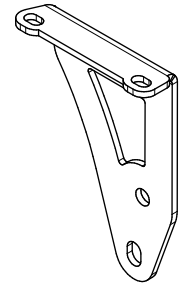
#MB1006-06 (DRIVER) MOUNTING BRACKET QTY 1
