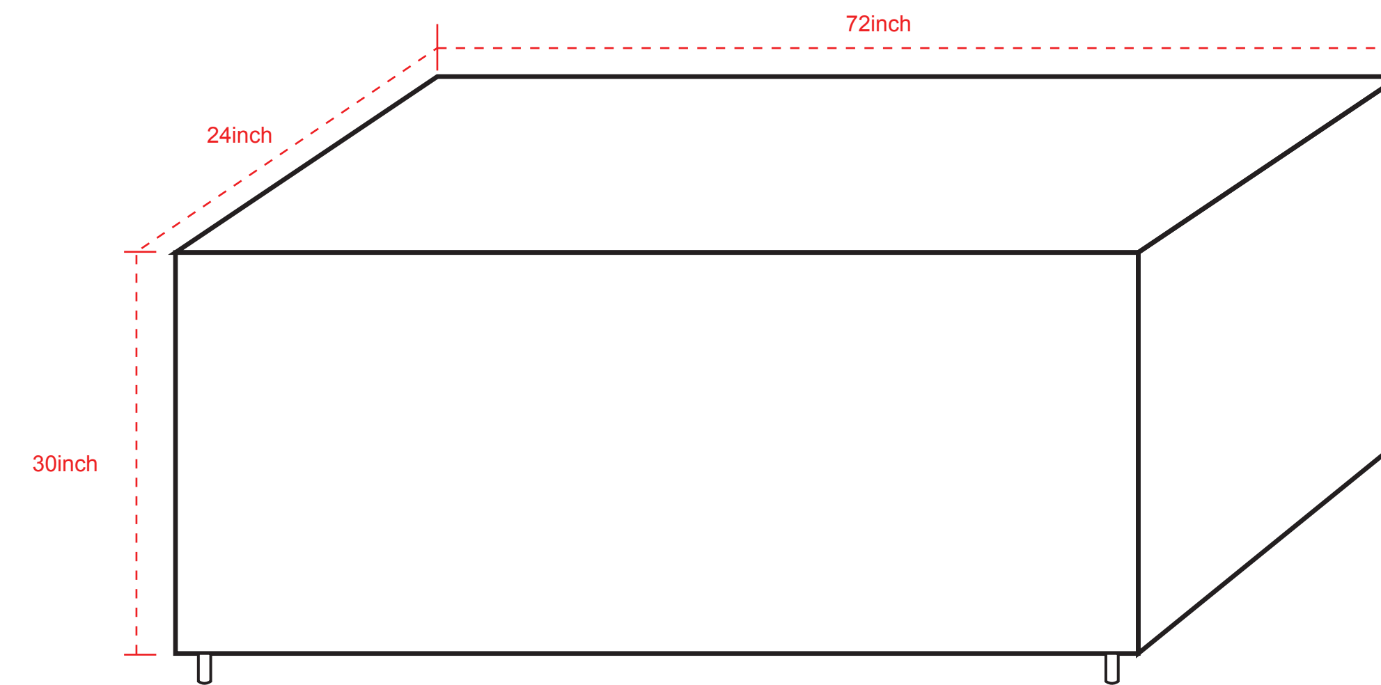
: Size C: 24"x72"x30 : ( 3D MMock up view )
