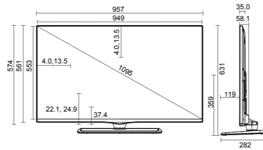
42F" 957 x 631 x 282 / 16.7kg VESA(mm): 400 x 400
