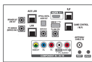
REAR JACK PANEL
