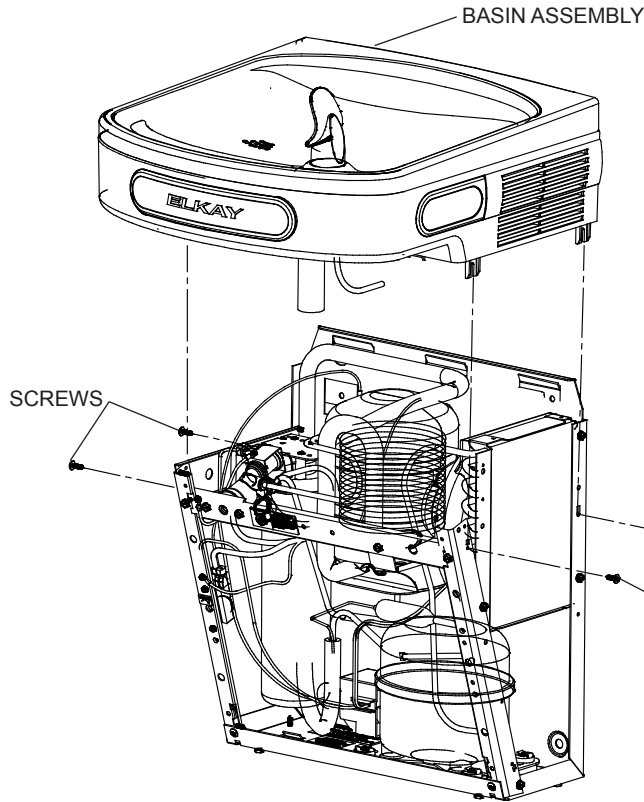
Basin Assembly Removal Fig. 4
