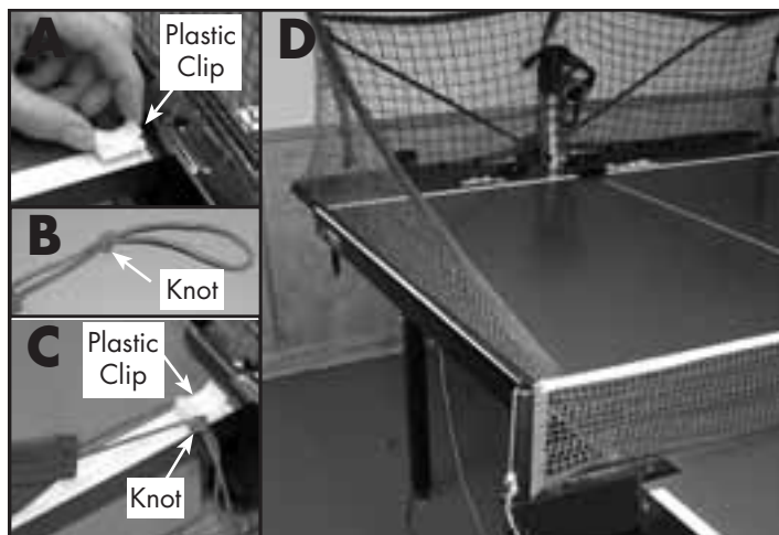
FIGURE 21 ATTACHING SIDE NETS WITH PLASTIC CLIPS (2040 ONLY)
