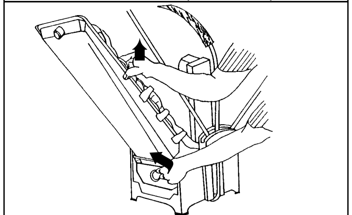
FIGURE 13 REMOVING BALL DAM (2040 ONLY)
