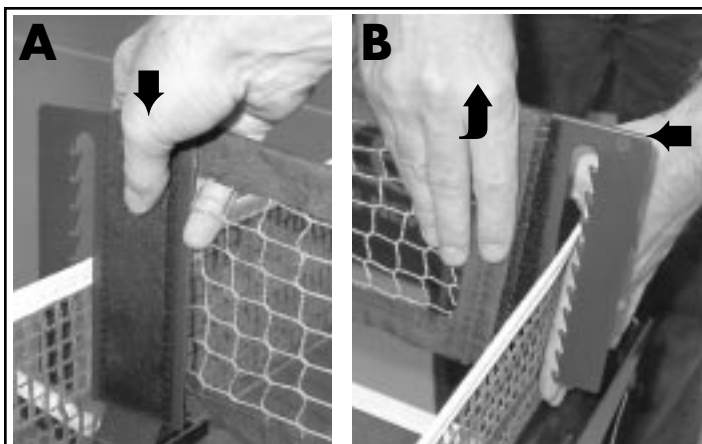
FIGURE 20 ATTACHING AND DETACHING THE SIDE NET (2040 ONLY)
