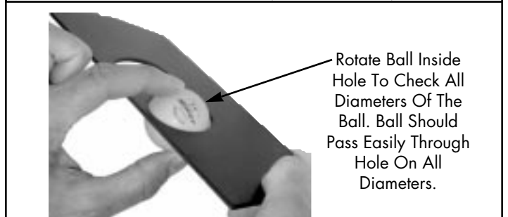
FIGURE 14 CHECKING BALL WITH BALL DAM (2040 ONLY)
