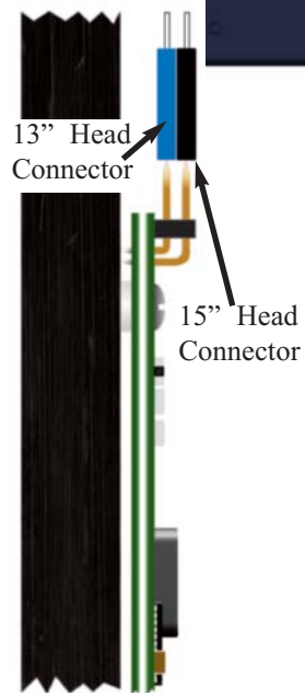
TI Board Side View
