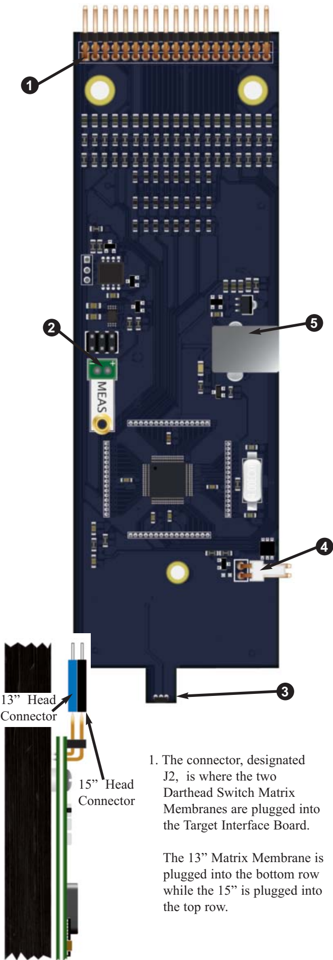
TI Board Side View
