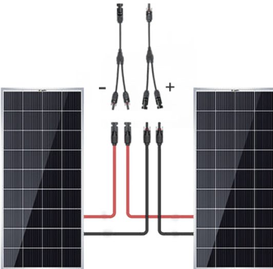
Parallel Connection
