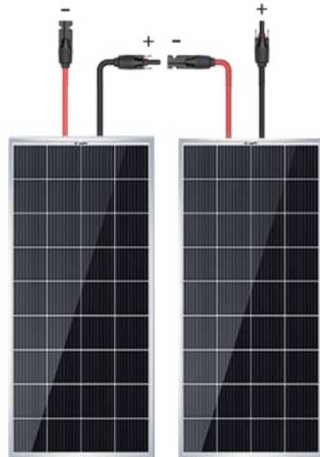
Electrical Connection
