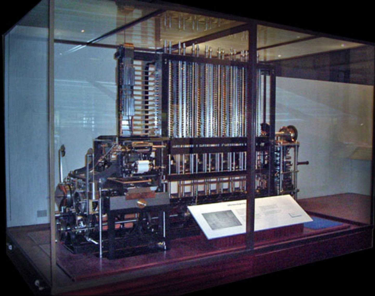
The London Science Museum's replica difference engine, built from Babbage's design. Photo by Joe D., Dorset, England. January 2005
