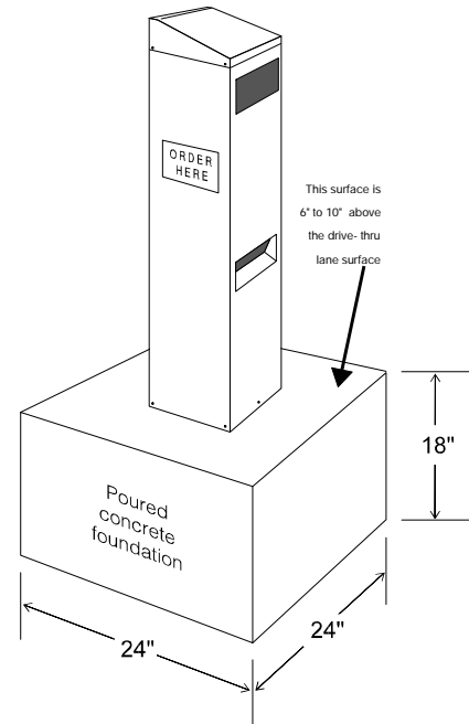
Figure 1. SPP2 Speaker Post on concrete foundation
