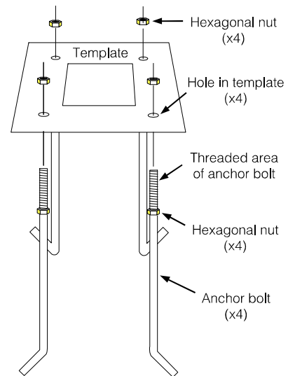
Figure 3. Assembly of anchor bolts with template
