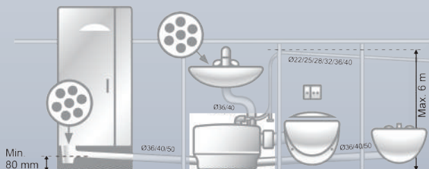
SOLOLIFT2 CWC-3 for wall-hung toilet, washbasin, bidet and a shower
