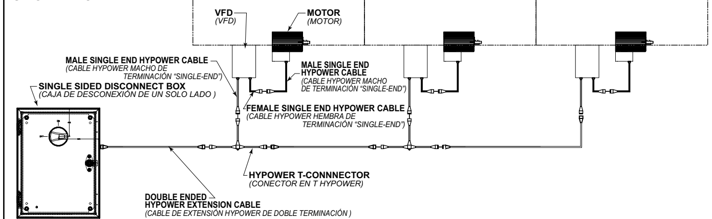
FIGURE 7C SINGLE DICONNECT
