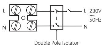
NA100/150 with remote switch
