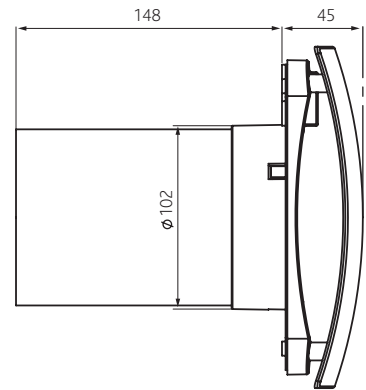
Side view of fan unit and grille
