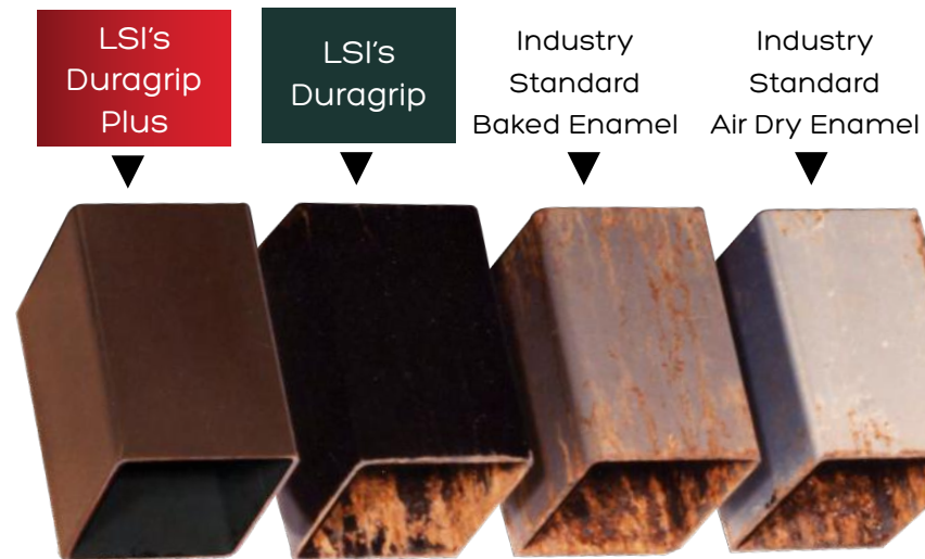
Poles After 1000hrs of Salt Spray Test
