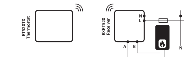
OPENTHERM
