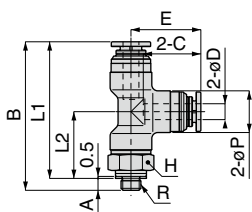
Metric thread
