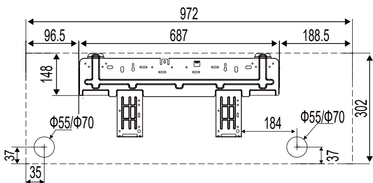
Mono-split : SMVH18B-4A2A3NG ( 18000 Btu )
