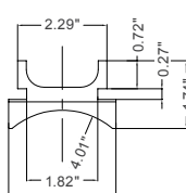
Round Pole Adapter (RPA) 4"
