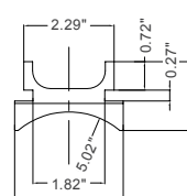
Round Pole Adapter (RPA) 5"
