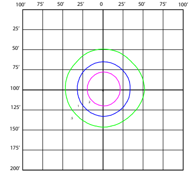
TYPE 5 - 100W 25' MOUNTING HEIGHT
