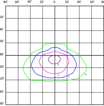
TYPE 4 - 75W 20' MOUNTING HEIGHT
