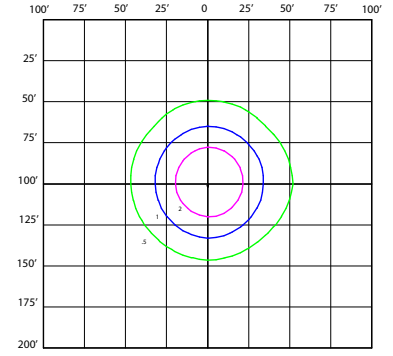
TYPE 5 - 100W 25' MOUNTING HEIGHT
