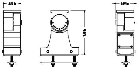
Adjustable Square Arm
