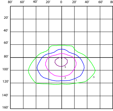
TYPE 4 - 75W 20' MOUNTING HEIGHT
