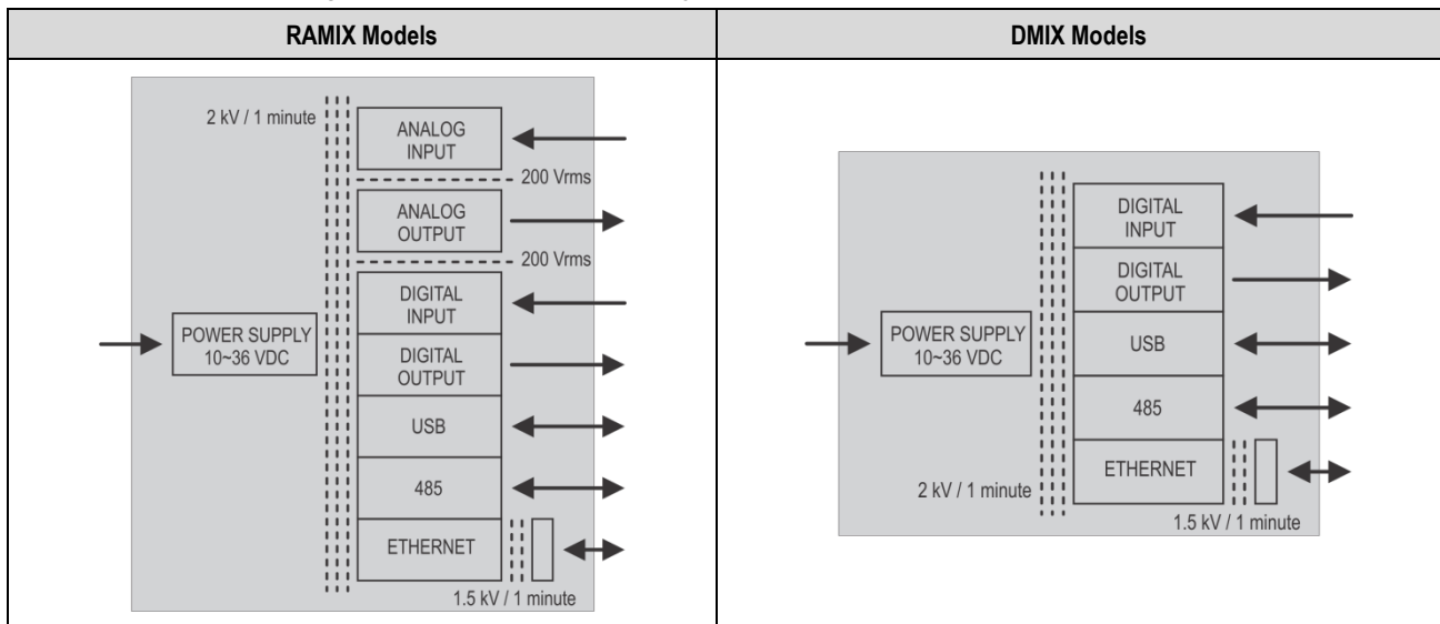
Fig. 12 – Electrical insulation
