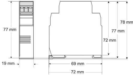
Figure 1 – Dimensions
