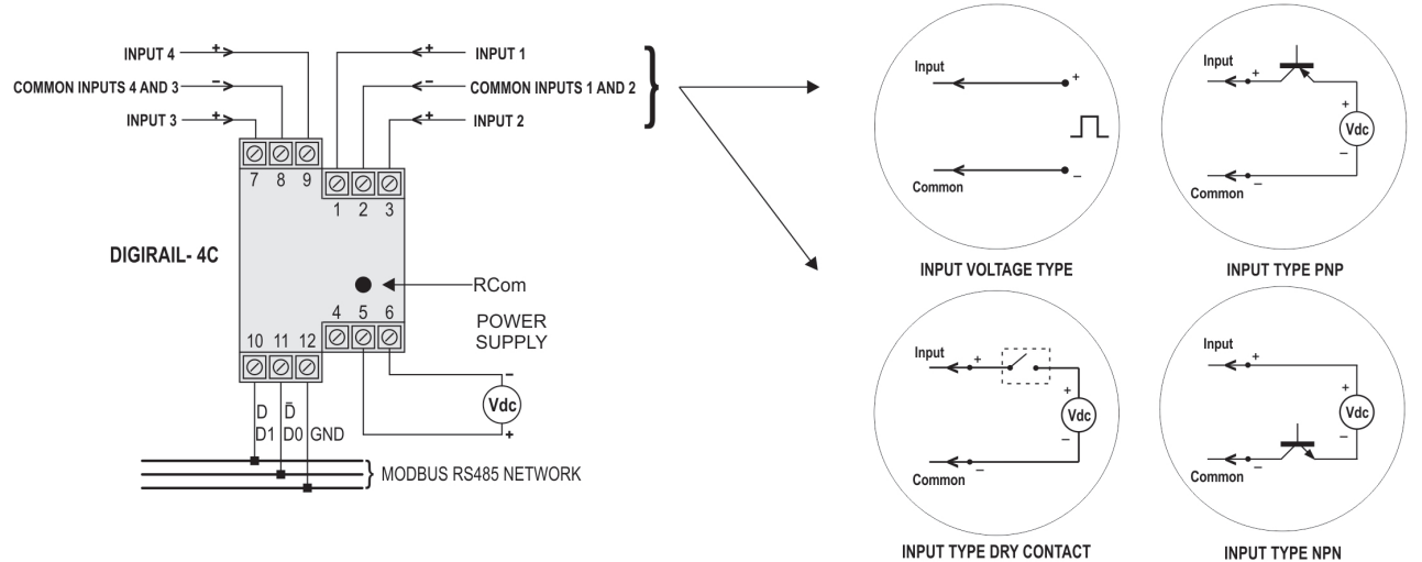
Figure 2 – Electrical Connections
