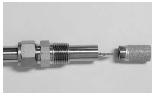
Figure 6-2 Sensor Exploded View for the RO120
