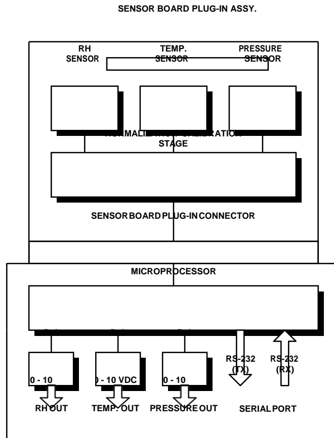
Figure 4-1 Basic Block Diagram, Probe Assy
