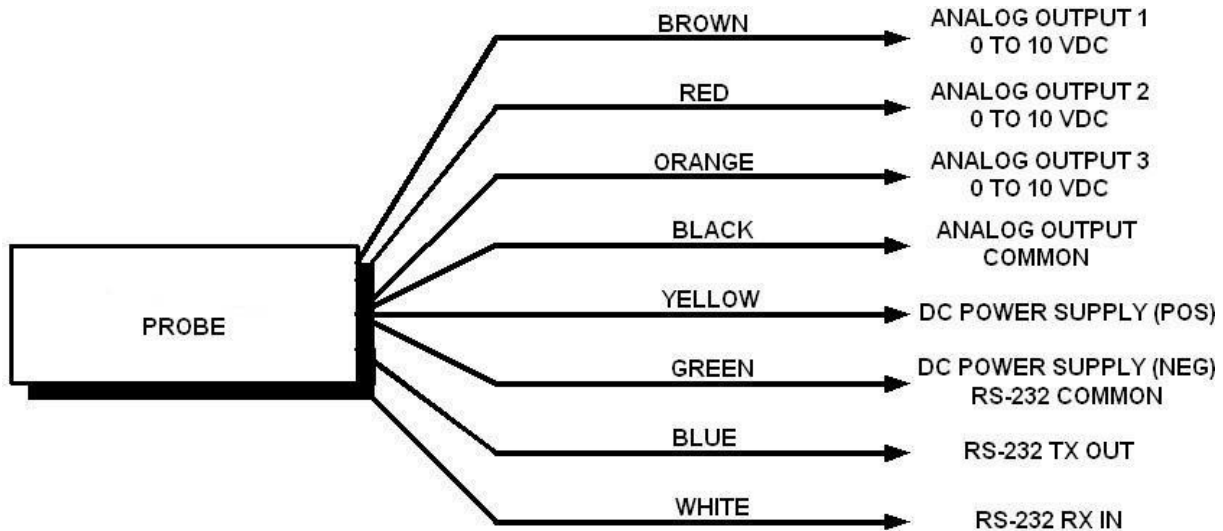
Figure 3-3a RO120 Series Probe (with Discrete Wires) Wiring Diagram
