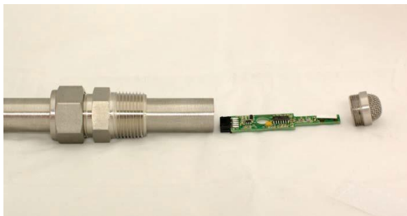
Figure 6-2 Sensor Exploded View for the RO120
