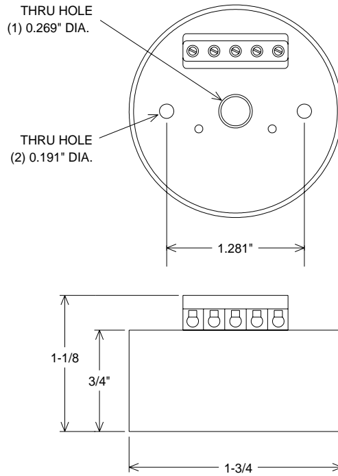
FIG. 3.2 - General Dimensions of 18-812
