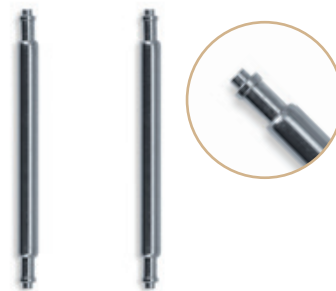
Shouldered WP0030YY
