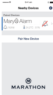
iOS Version
