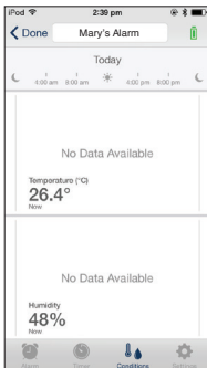
iOS Version
