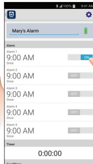
Android Version
