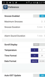
Android Version
