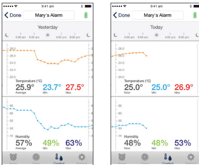
iOS Version
