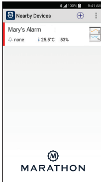
Android Version
