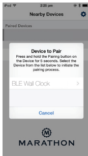
iOS Version
