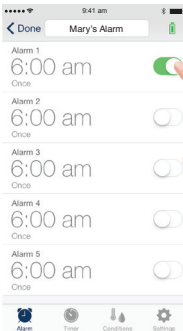
iOS Version
