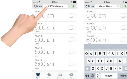
iOS Version
