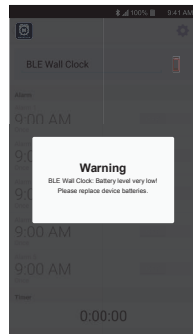
Android Version
