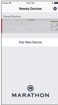
iOS Version
