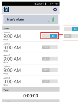
Android Version
