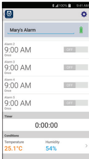
Android Version
