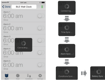
iOS Version
