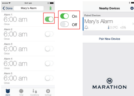
iOS Version
