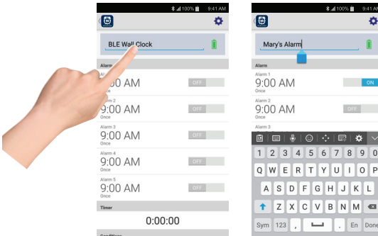
Android Version
