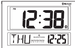
iOS Version
