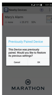
Android Version
