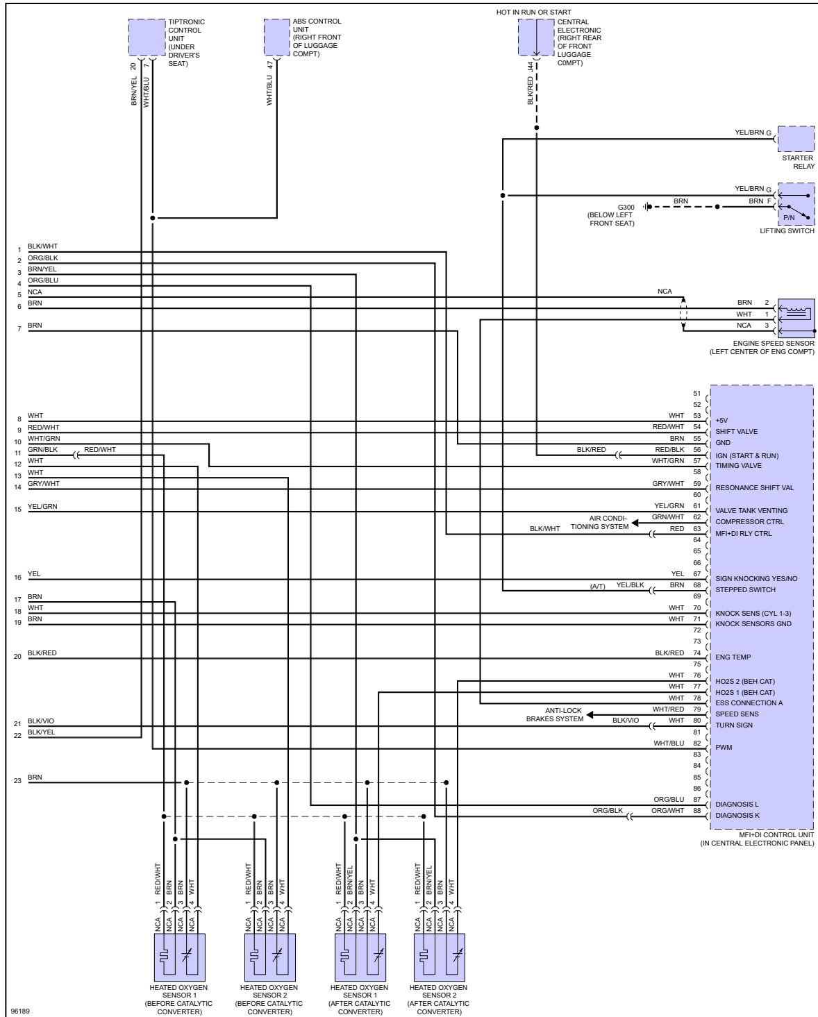
Fig 3: 3.6L, Engine Performance Circuits (3 of 3)
