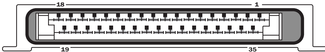
35 POSITION ECU PLUG PIN LAYOUT
