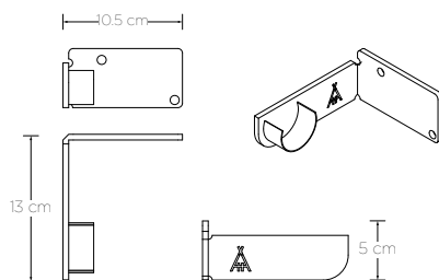
BASE PARED WALL BRACKETS
