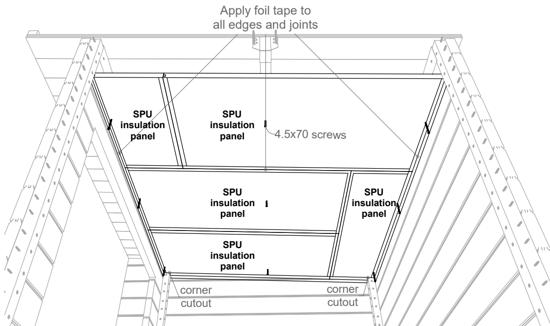
Scheme 3.5
