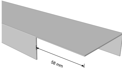
Scheme 10.2
