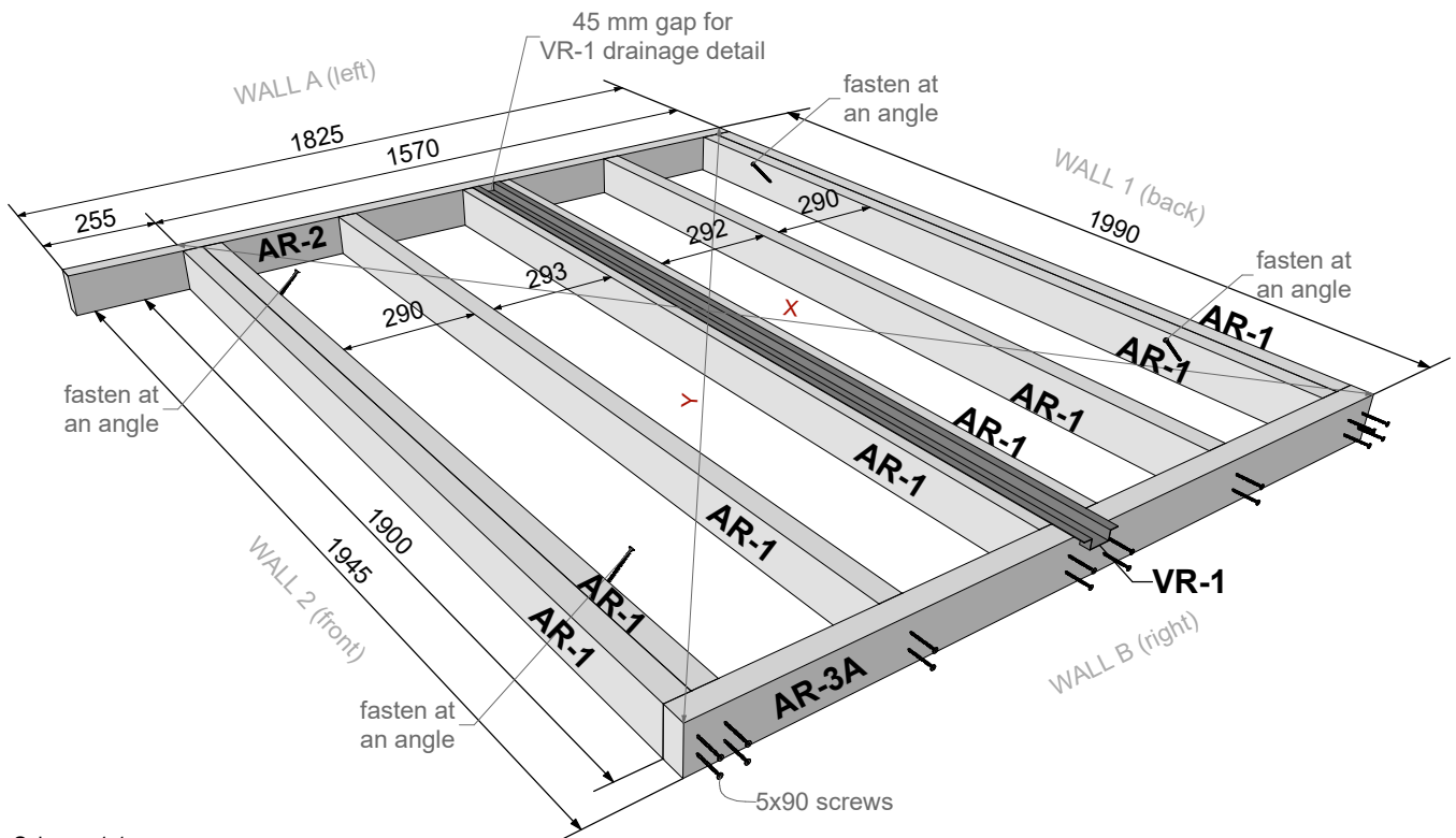
Scheme 1.1
