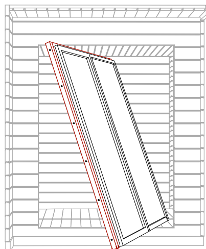
Scheme 5.2
