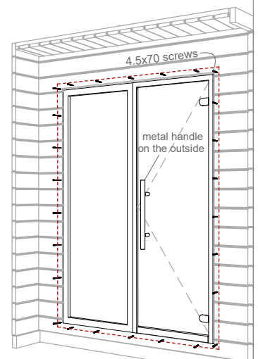
Scheme 5.3
