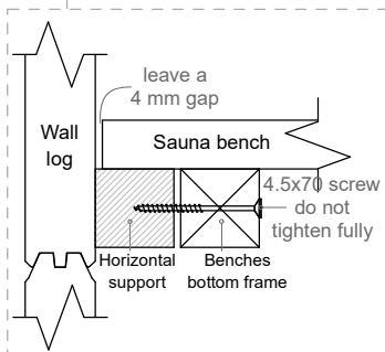
Scheme 8.3
