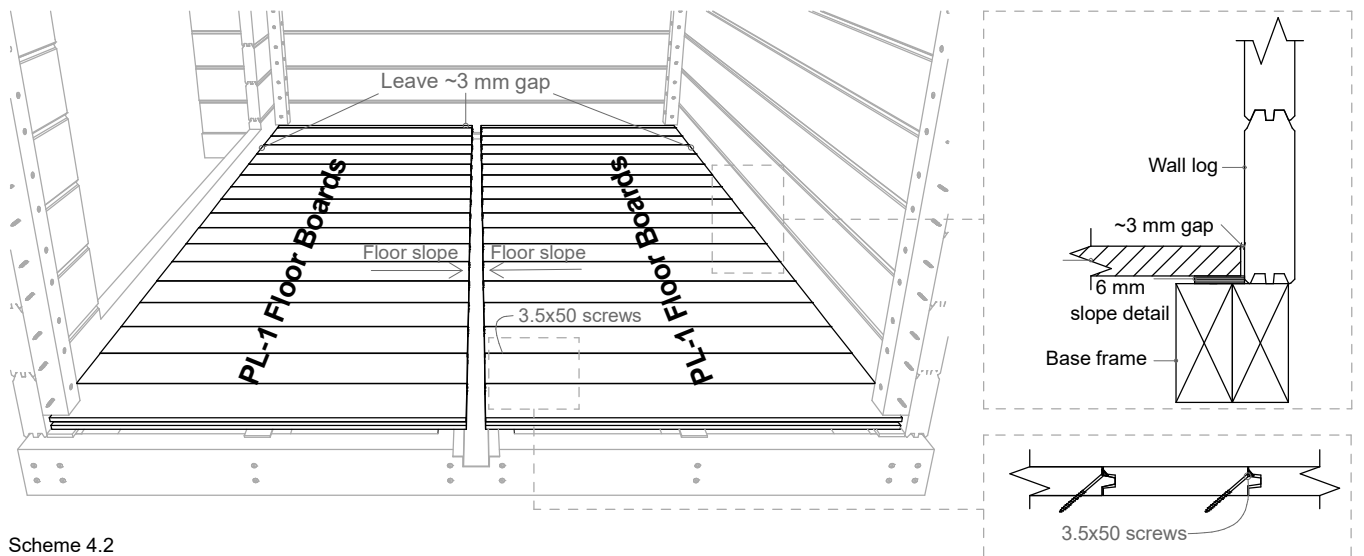
Scheme 4.2
