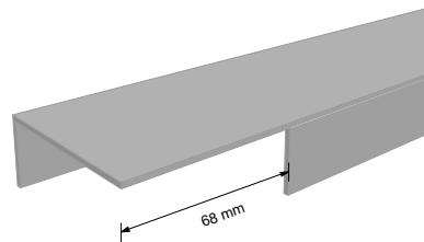
Scheme 10.3
