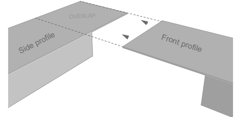
Scheme 10.4
