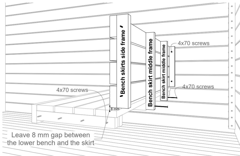
Scheme 8.2
