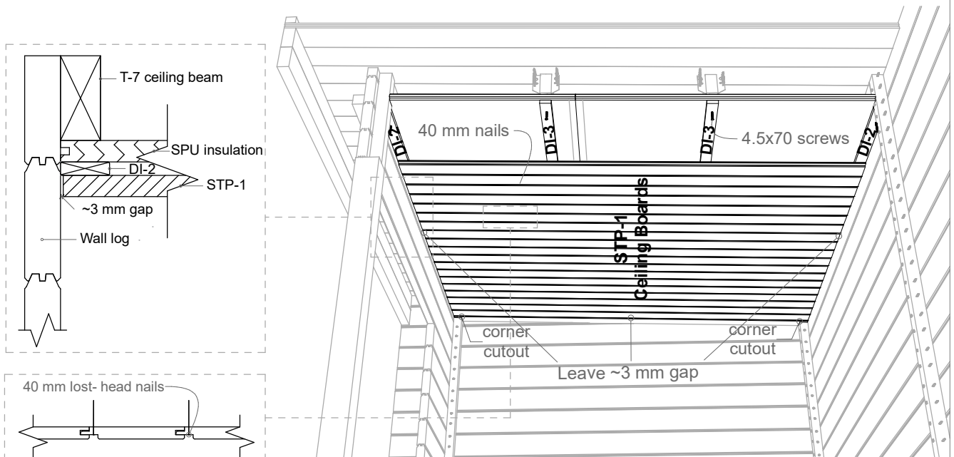
Scheme 3.10
