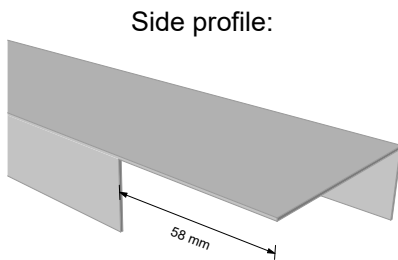
Scheme 10.2
