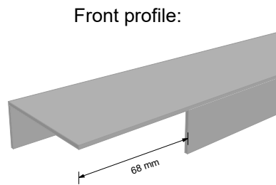
Scheme 10.3
