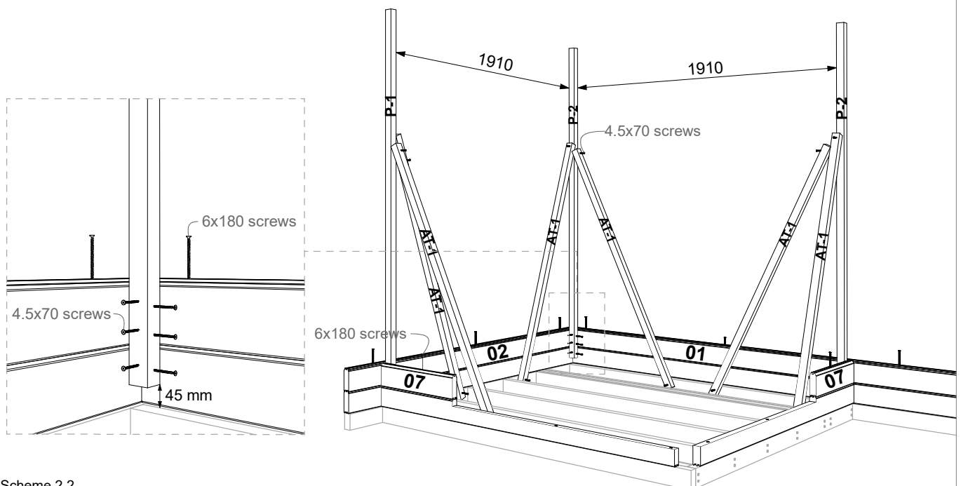
Scheme 2.2
