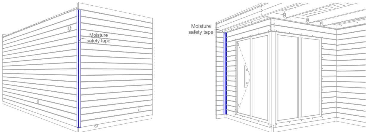
Scheme 7.2
