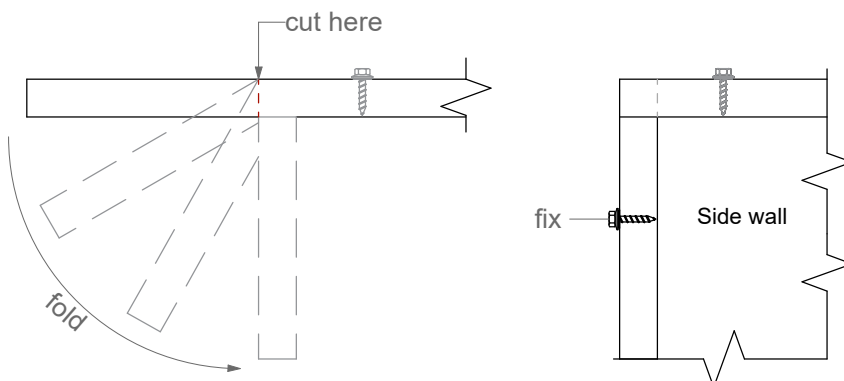
Scheme 10.7
