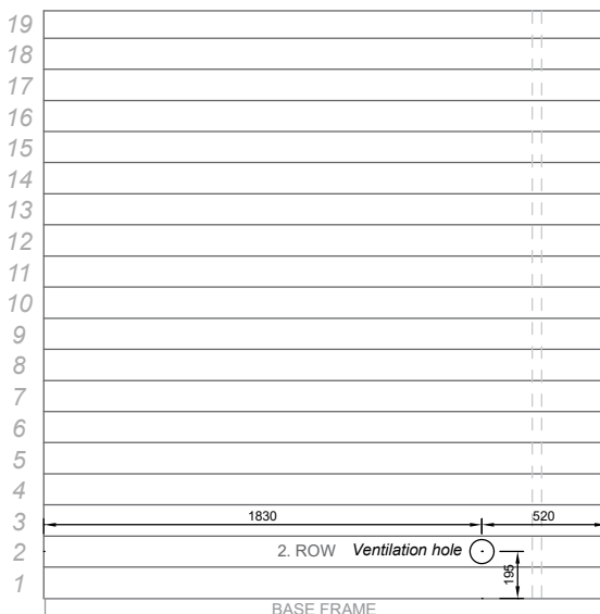
Scheme 6.1
