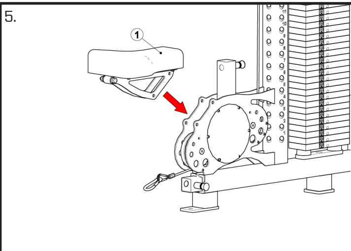
ALIGN LAT PULL SEAT TO BASE. (AS SHOWN)
