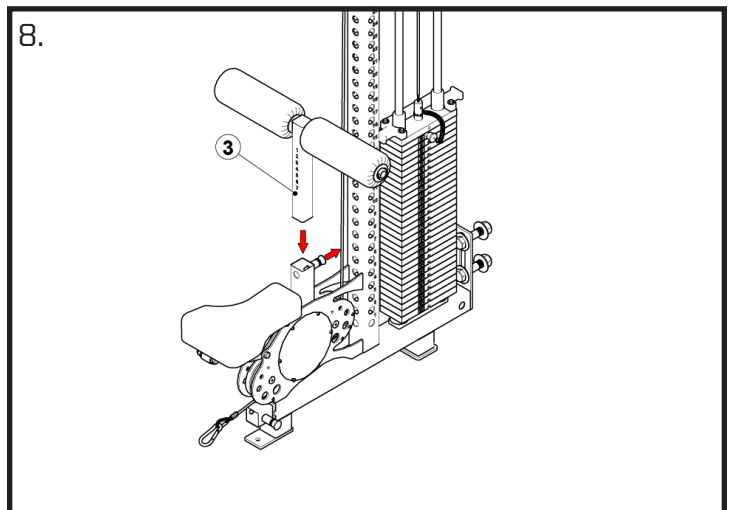
PULL POP PIN, THEN INSERT THIGH PAD POST. (AS SHOWN)
