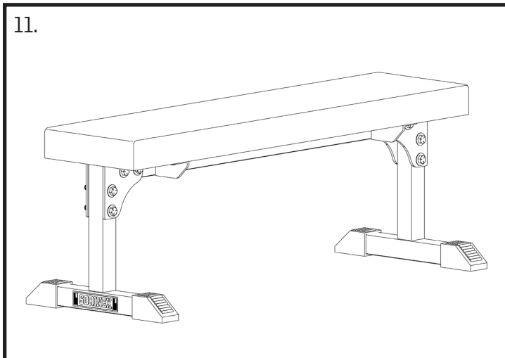
IF BENCH WOBBLER, LOOSEN 5/8" BOLTS. ALLOW BENCH TO SETTLE TO FLOOR, THEN RE-TIGHTEN BOLTS.
