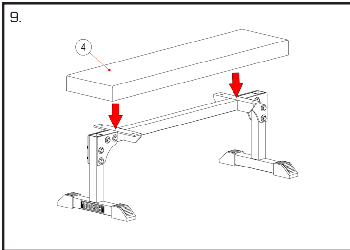
ALIGN PAD TO THE FOUR BOLT HOLES. (AS SHOWN)
