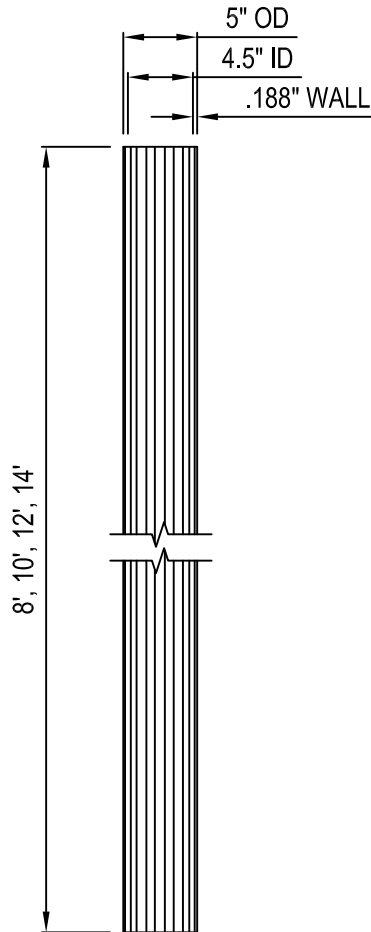
5" OD FLUTED POLE EXTRUDED ALUMINUM ALLOY 6005-T5
