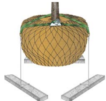
Tree Anchoring Systems: Deadman System - Plati-Mat & Strap (RF2RDMP & RF2RDMS)
