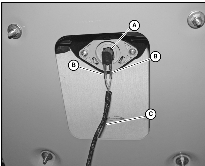
A. Seat switch B. Female spade connector C. Mower harness
