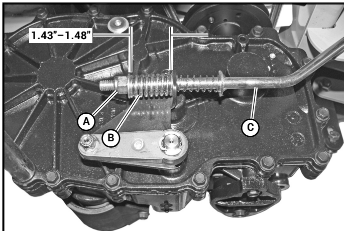
A. Nylock nut C. Park brake rod B. Park brake spring
