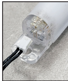
Fig. 1c. Molex will seat fully within the LED modules.
