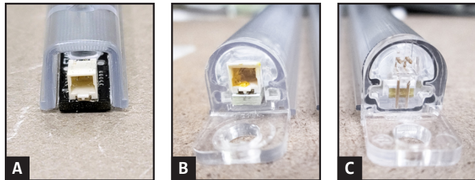
Fig. 1b. LED modules. All versions have a square receptacle for the molex connector. A & B have a white ring around the opening. C does not.
