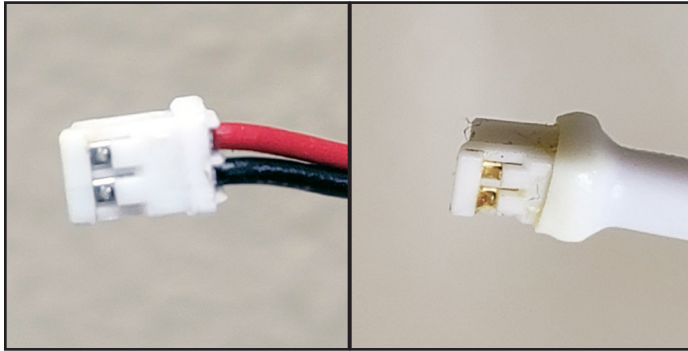
Fig. 1a. White molex-style connectors. All versions of this connector can be used on the LED modules shown.
