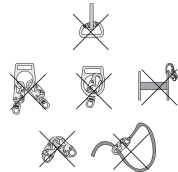
FIGURE 4 - INAPPROPRIATE CONNECTIONS
