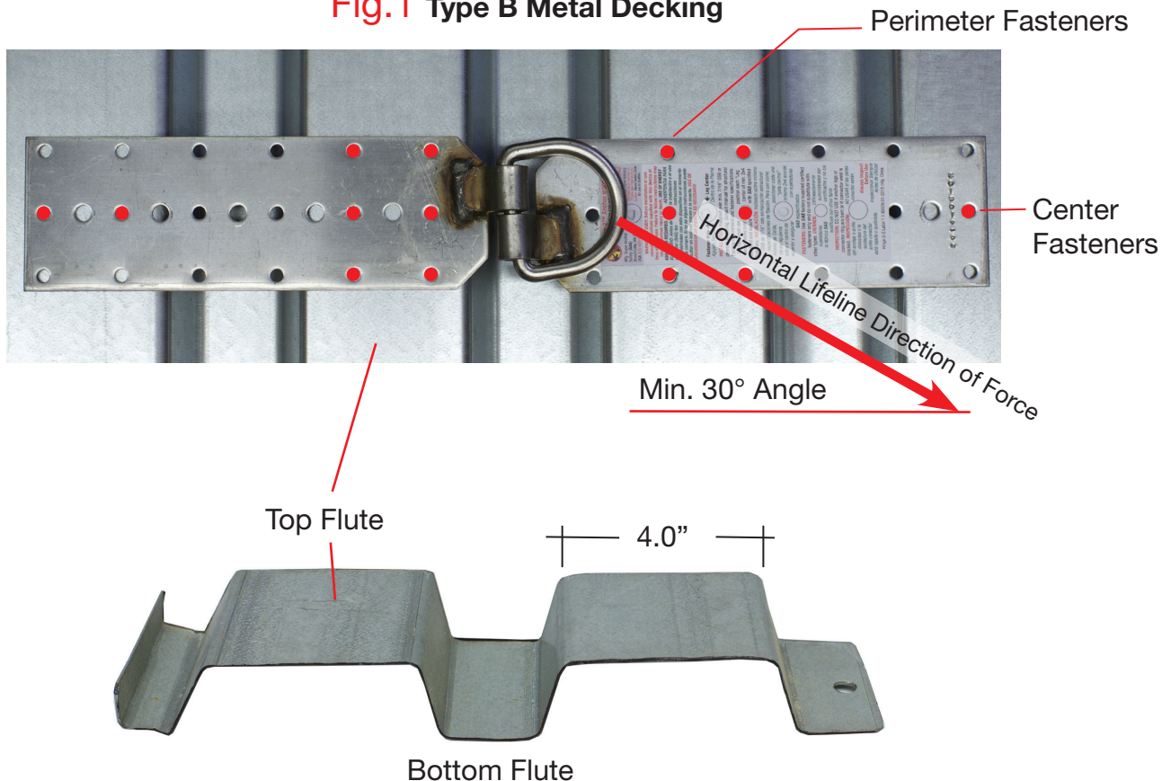
Fig.1 Type B Metal Decking
