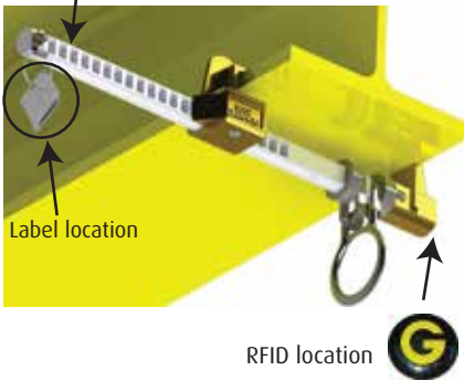
Date of Manufacture engraved on Aluminum Bar
