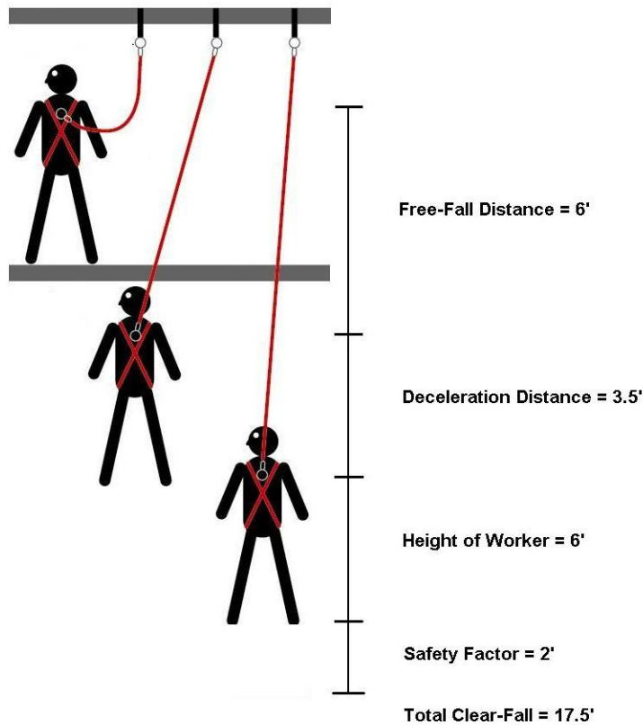
Figure 2.1: Clear-Fall Diagram
