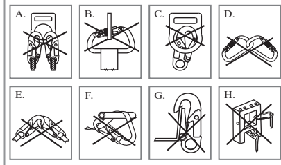
Figure 5 - Inappropriate Connections
