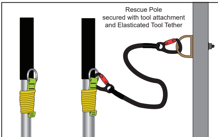
FIGURE 10 - RESCUE POLE TOOL TETHER/LANYARD
